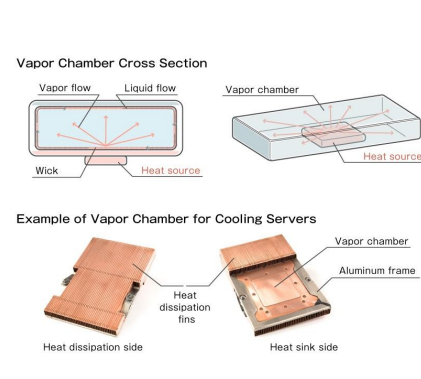
Vapor Chamber
