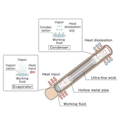
Heat Pipe
